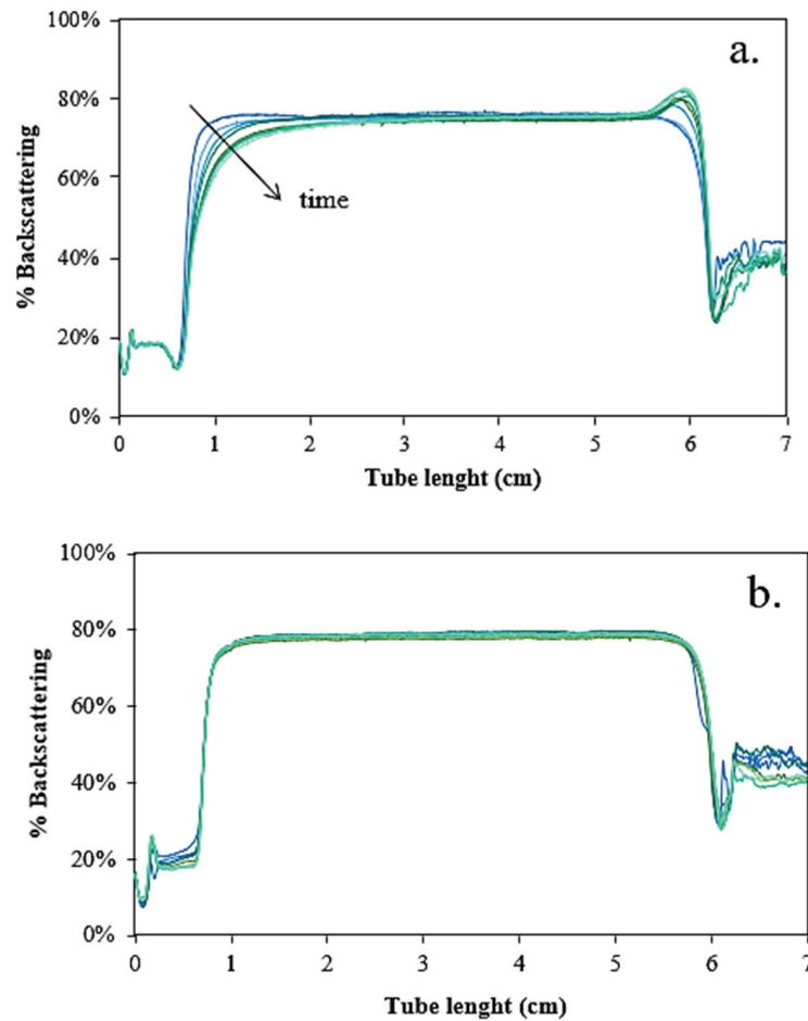
Figure 3. Back scattering profiles (%BS vs. tube length) of mono- (a) and bilayer (b) chia O/W emulsions during refrigerated storage.
